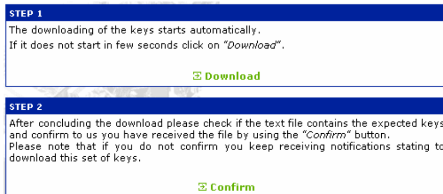
Figure 4 - "Downloading" Page
